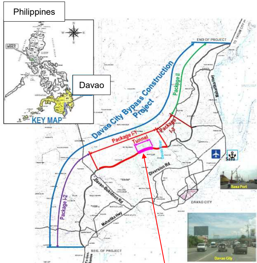
Davao City Bypass Construction Project (Total length – 10.7km) ※ Target section (Tunnel – 2.3km)
